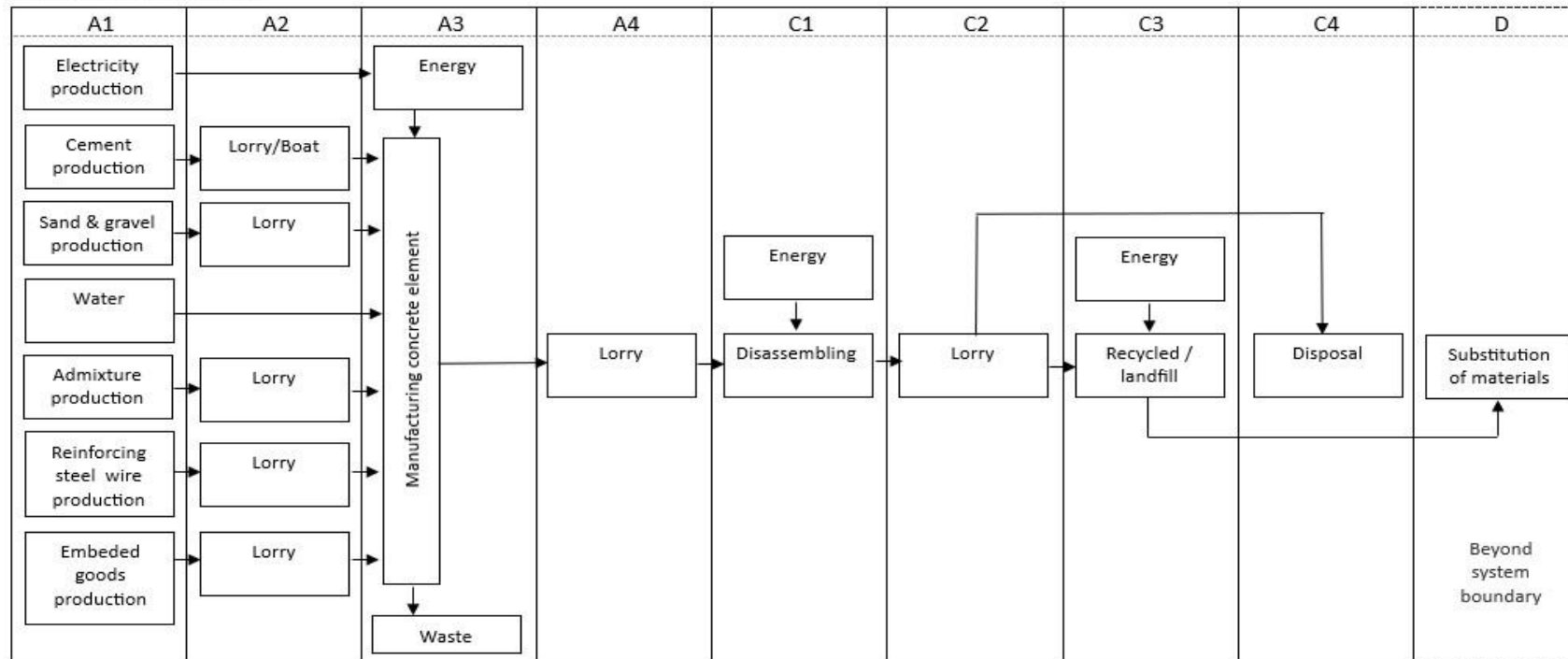
Flowchart over production
